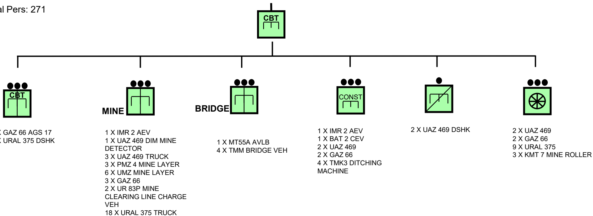
MT55A AVLB
