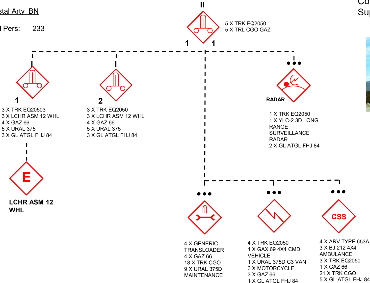
YLC-2 3D LONG RANGE SURVEILLANCE RADAR
